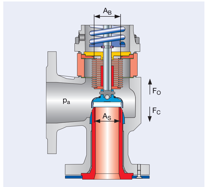
Type 546
